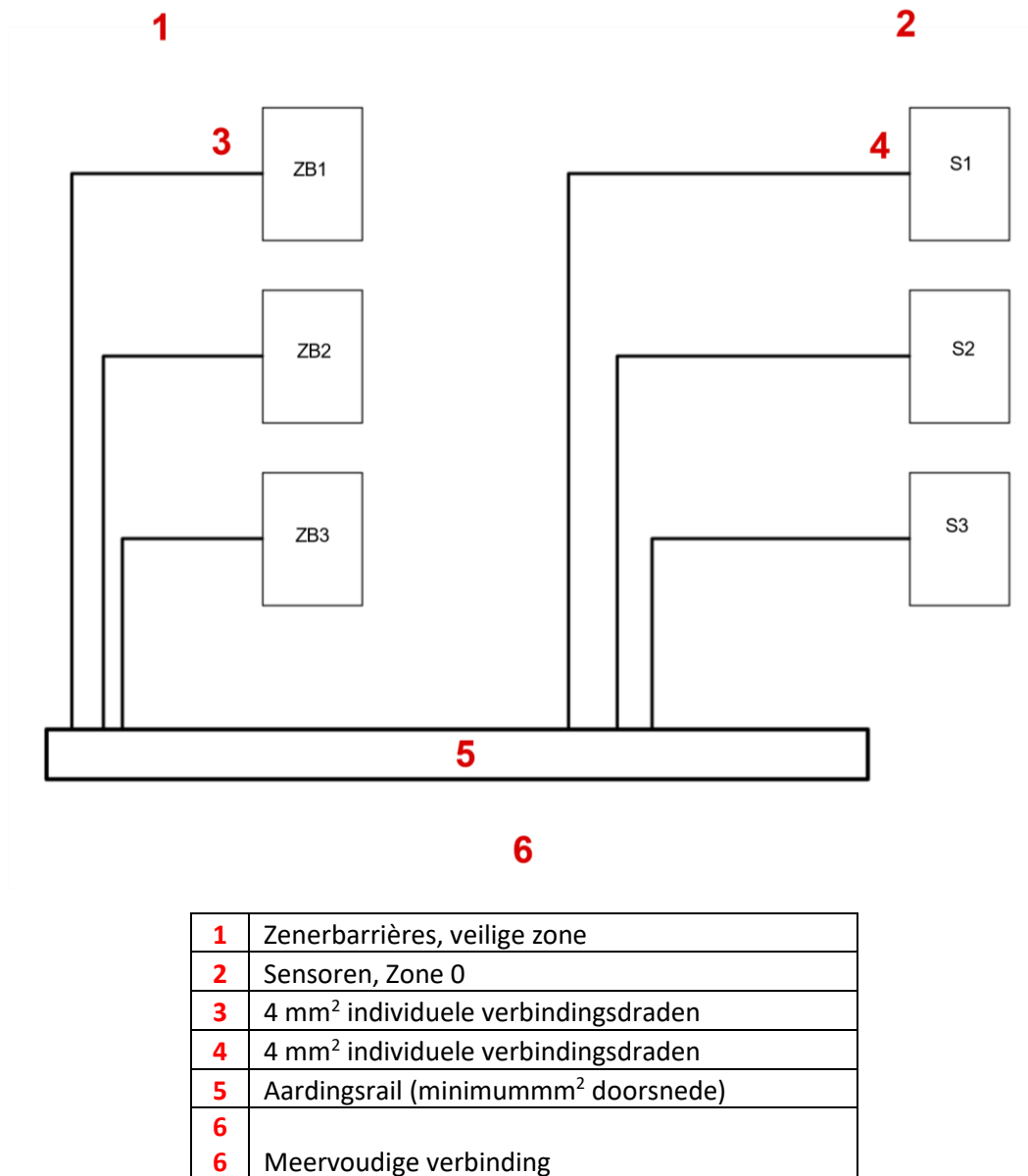
Figuur 15: Hybride of multi-drop verbinding
